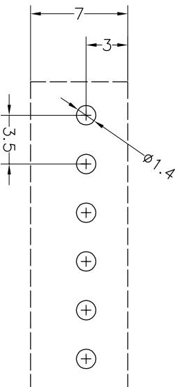
Recommended P.C.B. Layout(Top Side)
